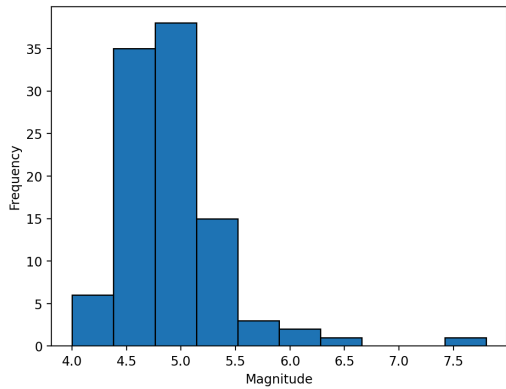
Magnitude Distribution
